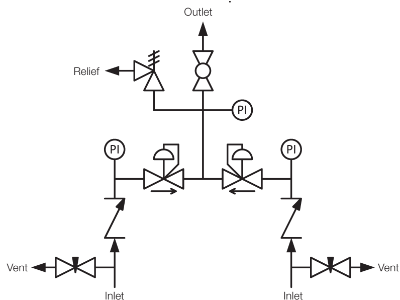
Fig. 19 SCO P&amp;ID without Outlet Pressure Regulator
