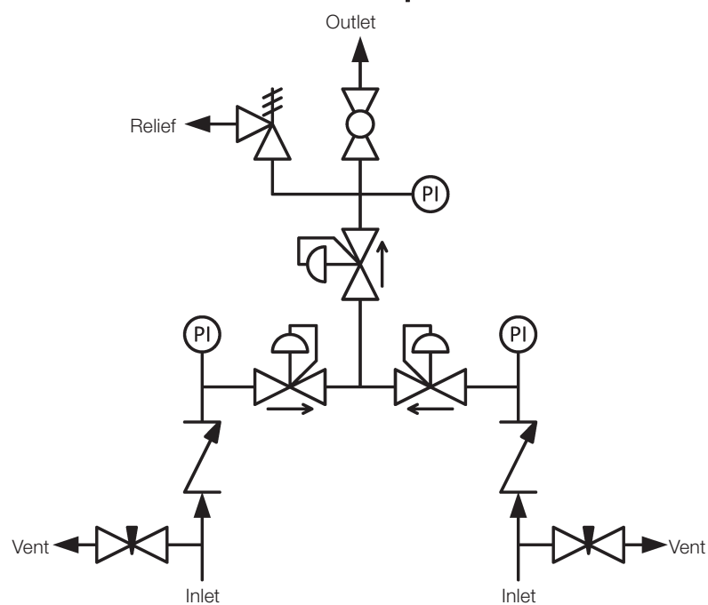
Fig. 20 SCO P&amp;ID with Outlet Pressure Regulator
